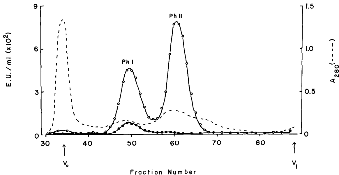
Fig.1. Chromatogram of untreated human brain extract on Sephacryl S-300. Assay was with 20 \mu l aliquots for 1 h at 37°C. Total phosphorylase activity (○); phosphorylase a (●); A_{280} -values (---).
