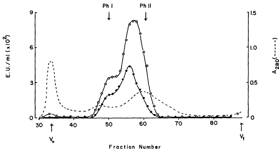
Fig.3. Sephacryl S-300 chromatogram of human brain extract treated with phosphorylase kinase. Assay was with 20 \mu l aliquots for 1 h at 37°C. Total phosphorylase activity (○); phosphorylase \alpha (●).
